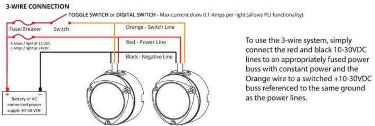
Figure 1: Kraken wiring diagram. Basic installation.
